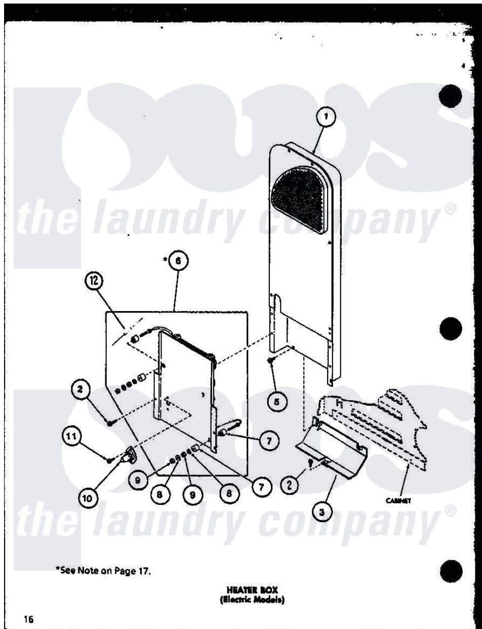
Amana Residential Amana LE2902 (BOM: P7804825W) Dryer Parts Diagram 03 - HEATER BOX (ELECTRIC MODELS)
