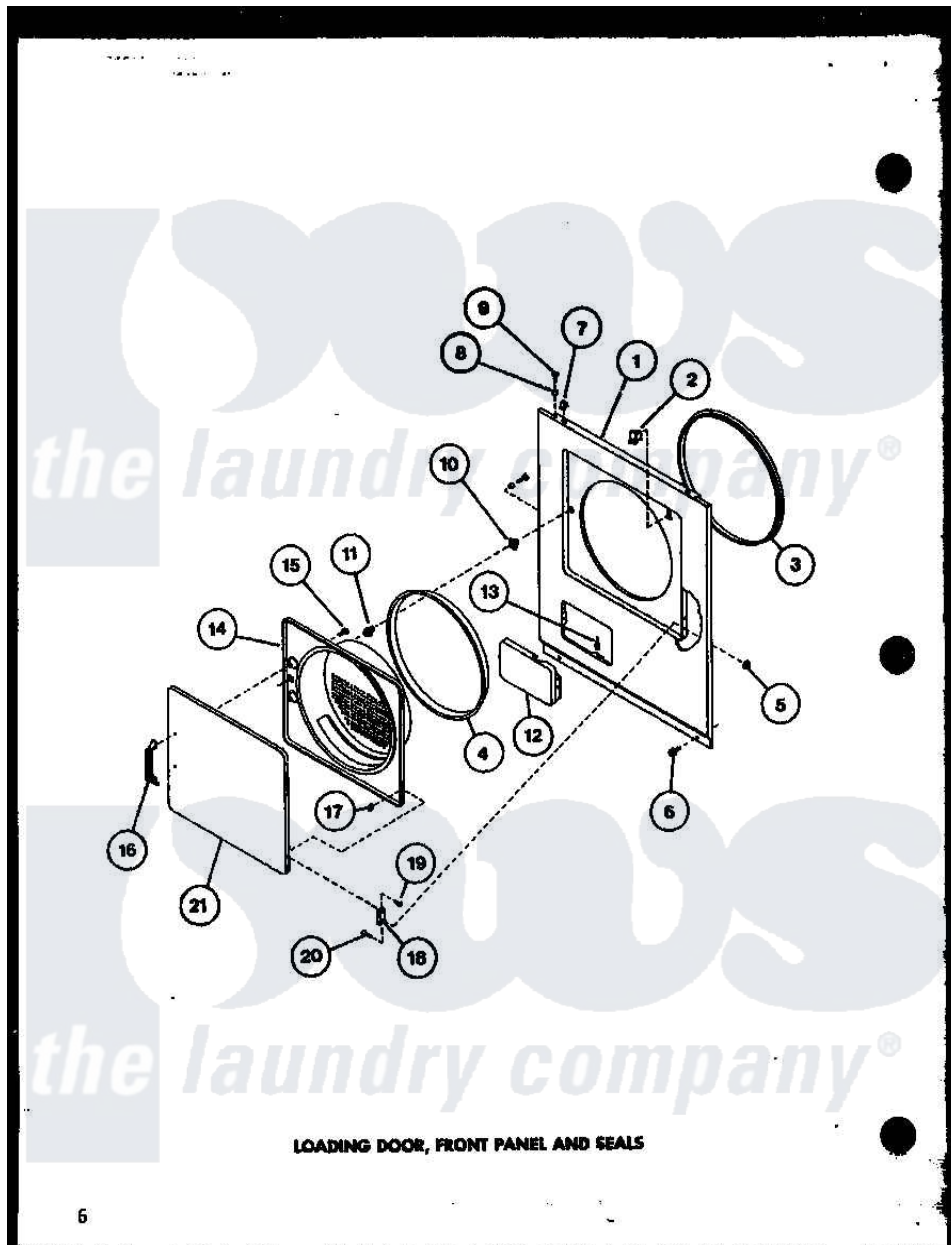
Amana Residential Amana LE2902 (BOM: P7804825W) Dryer Parts Parts Diagram 04 - LOADING DOOR Click on the part number to view part
