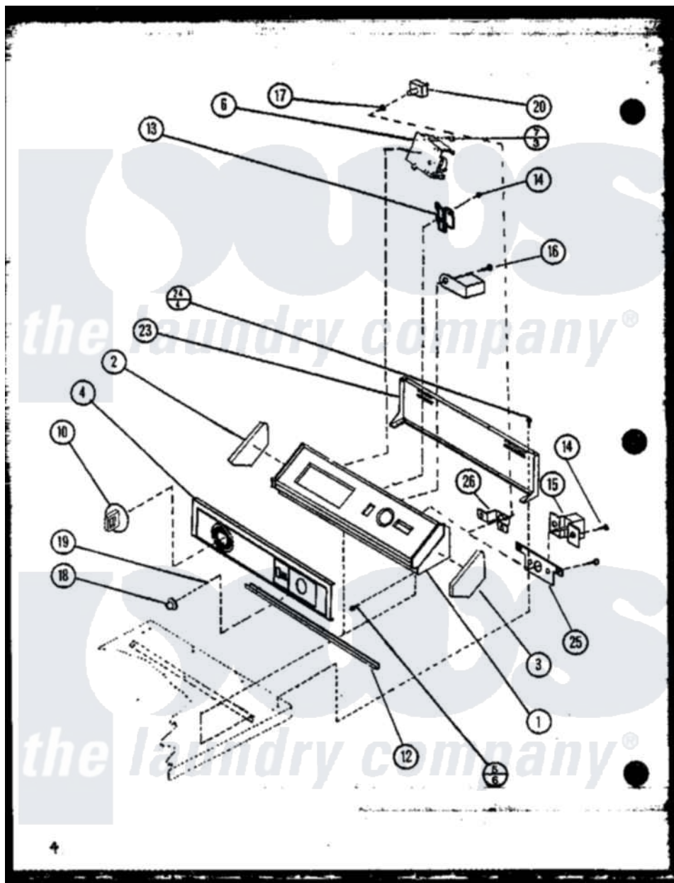
Amana Residential Amana LE3502L (BOM: P1118307W L) Dryer Parts Parts Diagram 07 - PAGE 1
