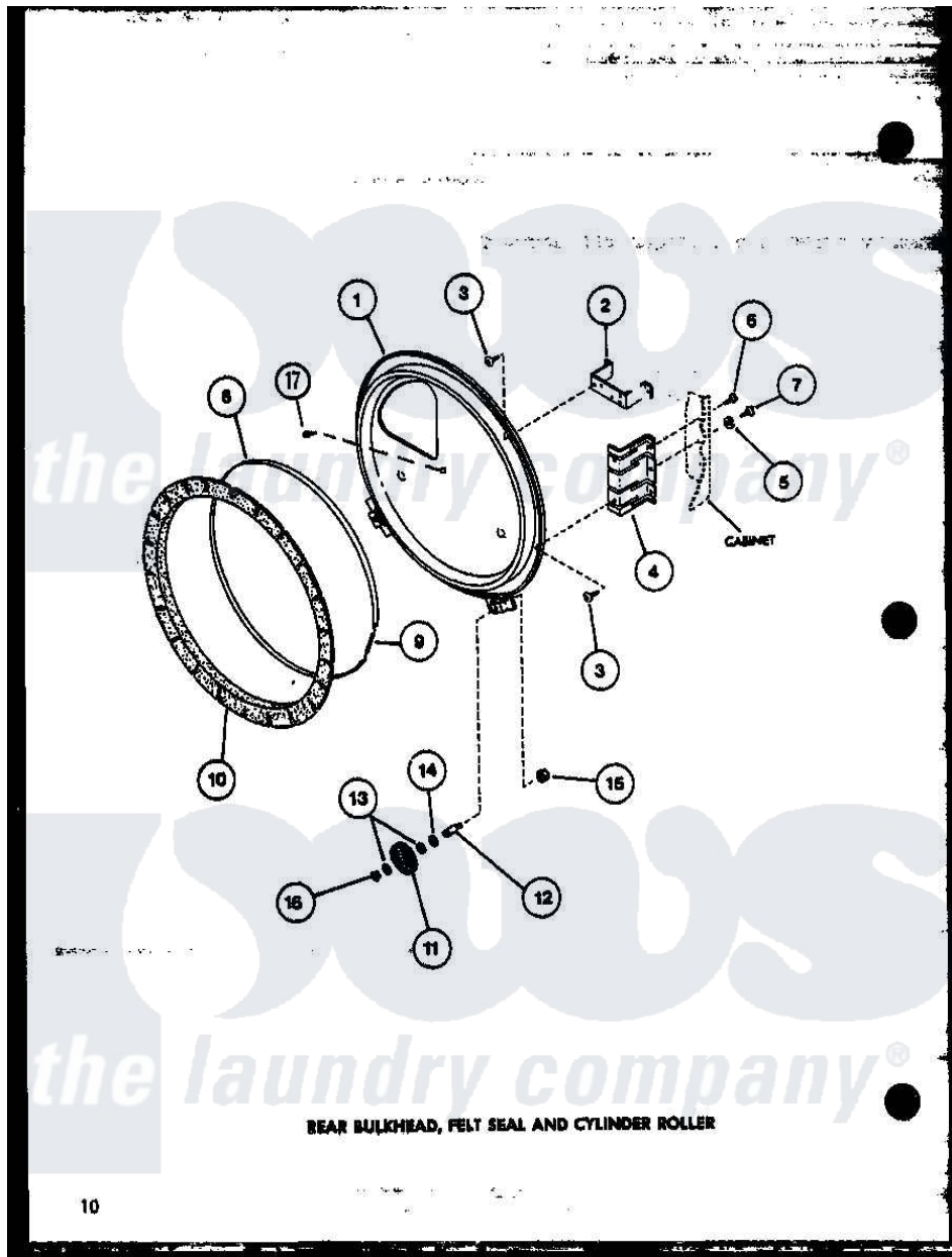
Amana Residential Amana LE3502L (BOM: P1118307W L) Dryer Parts Parts Diagram 08 - REAR BULKHEAD Click on the part number to view part
