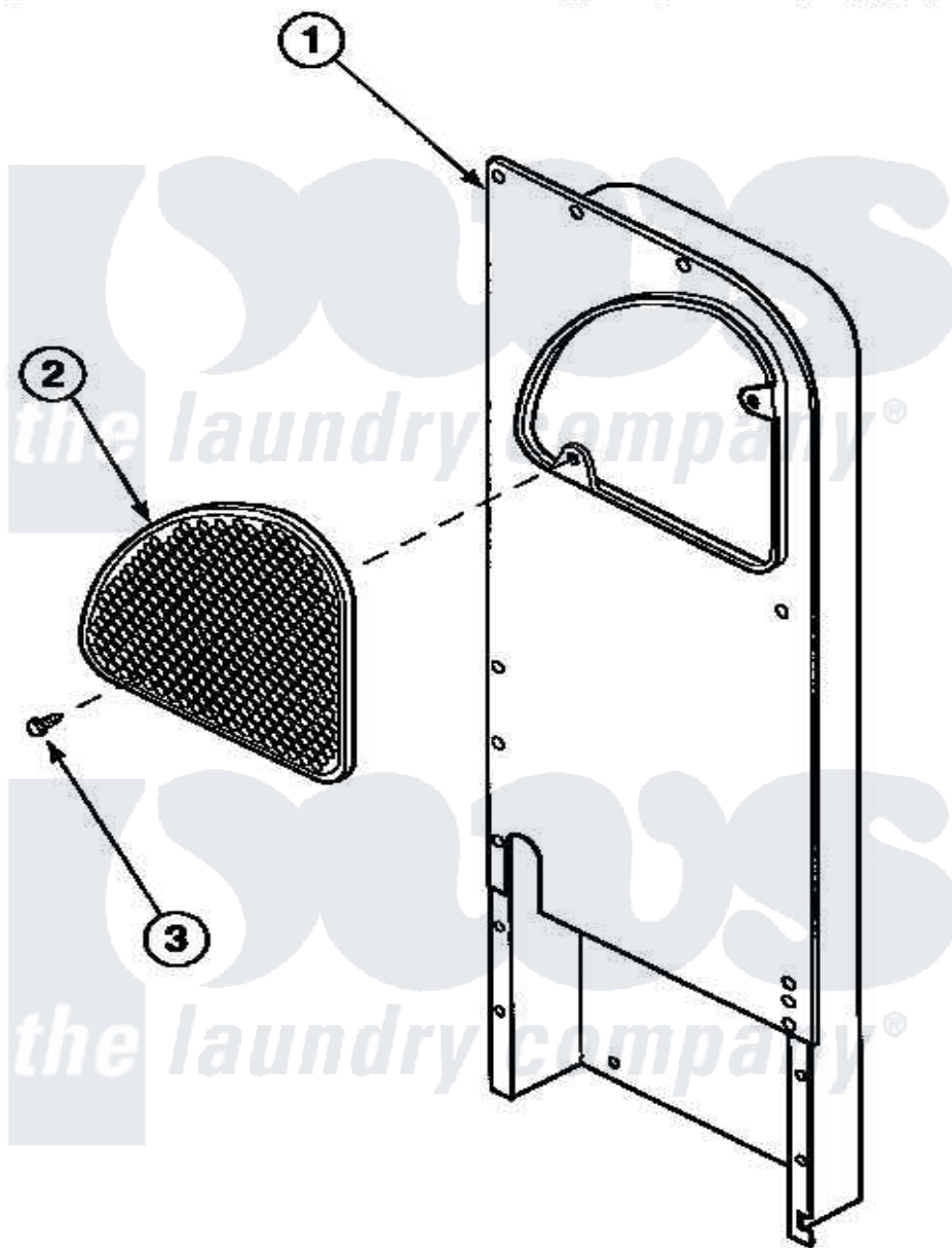
Amana Residential Amana LE7111WB (BOM: PLE7111WB) Dryer Parts Parts Diagram 12 - HEATER BOX ASSY REPLACEMENT
