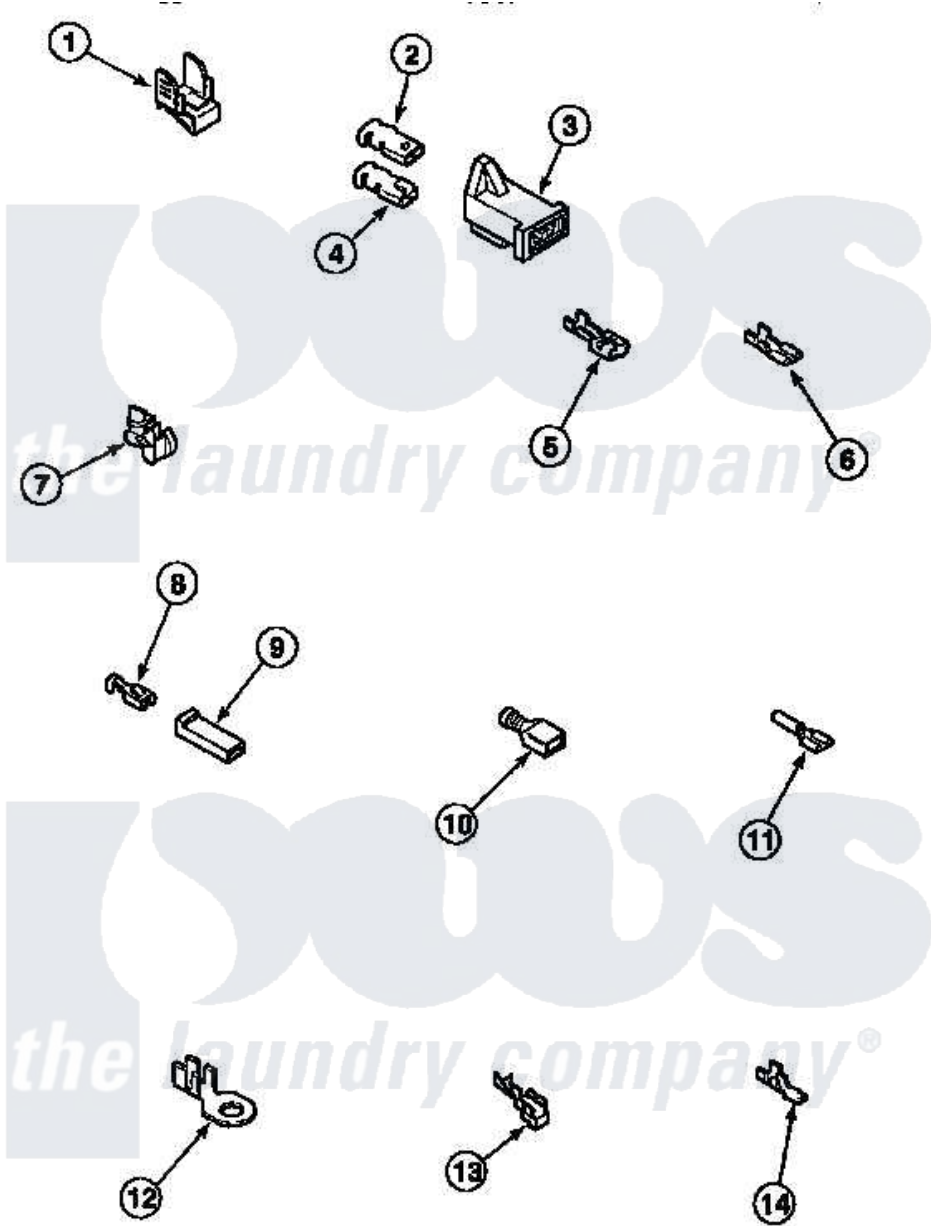
Amana Residential Amana LE7111WB (BOM: PLE7111WB) Dryer Parts Parts Diagram 21 - TERMINALS Click on the part number to view part
