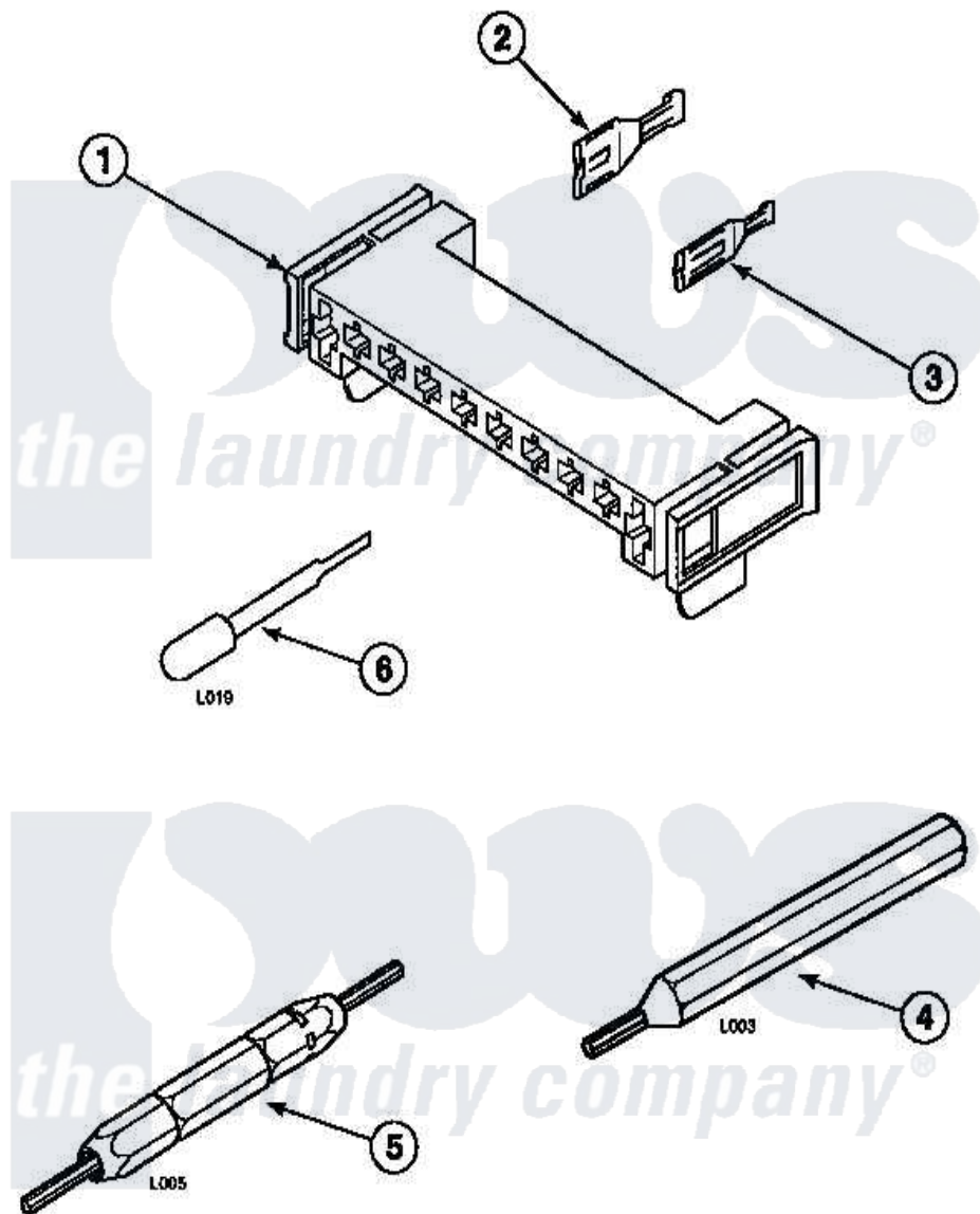
Amana Residential Amana LE7111WM (BOM: PLE7111WM) Dryer Parts Parts Diagram 16 - Page 21 Click on the part number to view part
