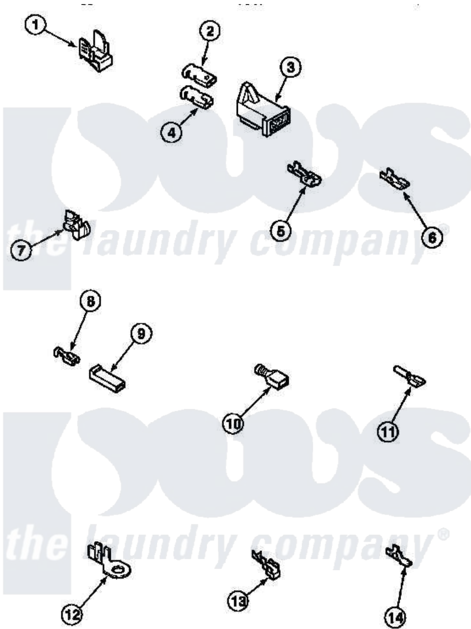
Amana Residential Amana LE7111WM (BOM: PLE7111WM) Dryer Parts Parts Diagram 21 - TERMINALS Click on the part number to view part
