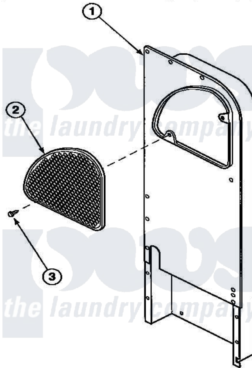
Amana Residential Amana LE7121LM (BOM: PLE7121LM) Dryer Parts Parts Diagram 12 - HEATER BOX ASSY REPLACEMENT
