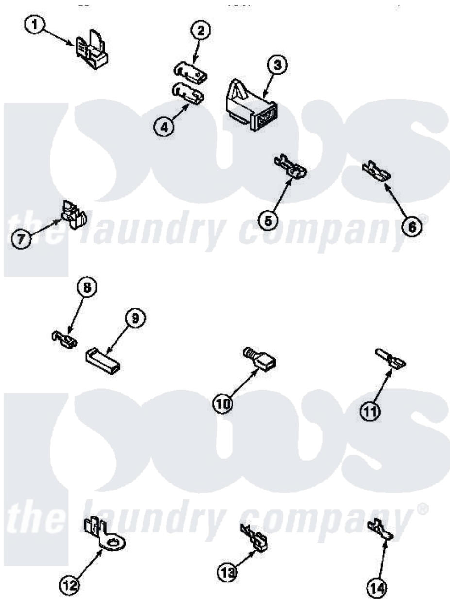
Amana Residential Amana LE8207L2 (BOM: PLE8207L2) Washer Parts Parts Diagram 21 - TERMINALS Click on the part number to view part
