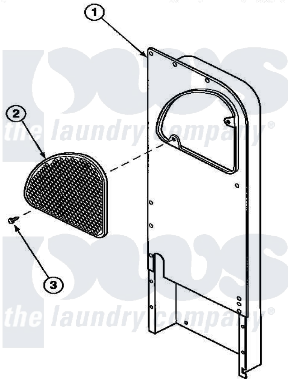
Amana Residential Amana LE8207L3 (BOM: PLE8207L3) Washer Parts Parts Diagram 12 - HEATER BOX ASSY REPLACEMENT
