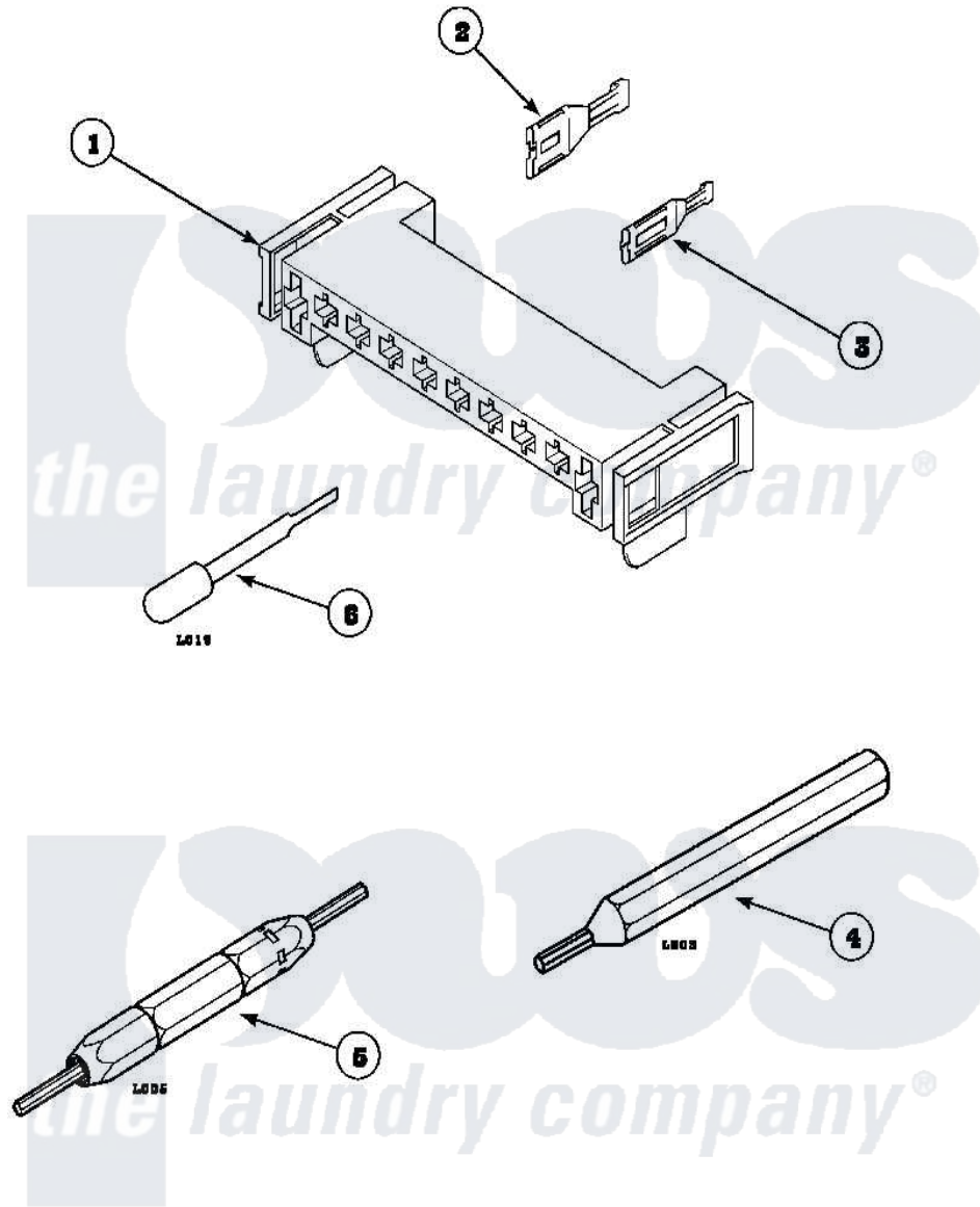
Amana Residential Amana LE8207W2B (BOM: PLE8207W2 B) Dryer Parts Parts Diagram 10 - Page 14 Click on the part number to view part
