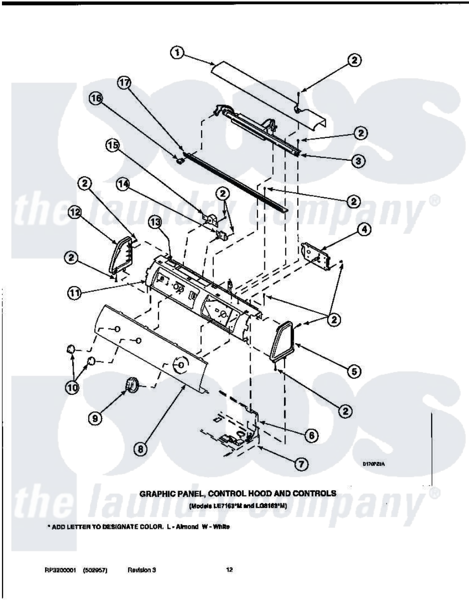
Amana Residential Amana LE8407L2 (BOM: PLE8407L2) Dryer Parts Parts Diagram 08 - GRAPHIC PANEL, CONTROL HOOD AND CONTROLS
