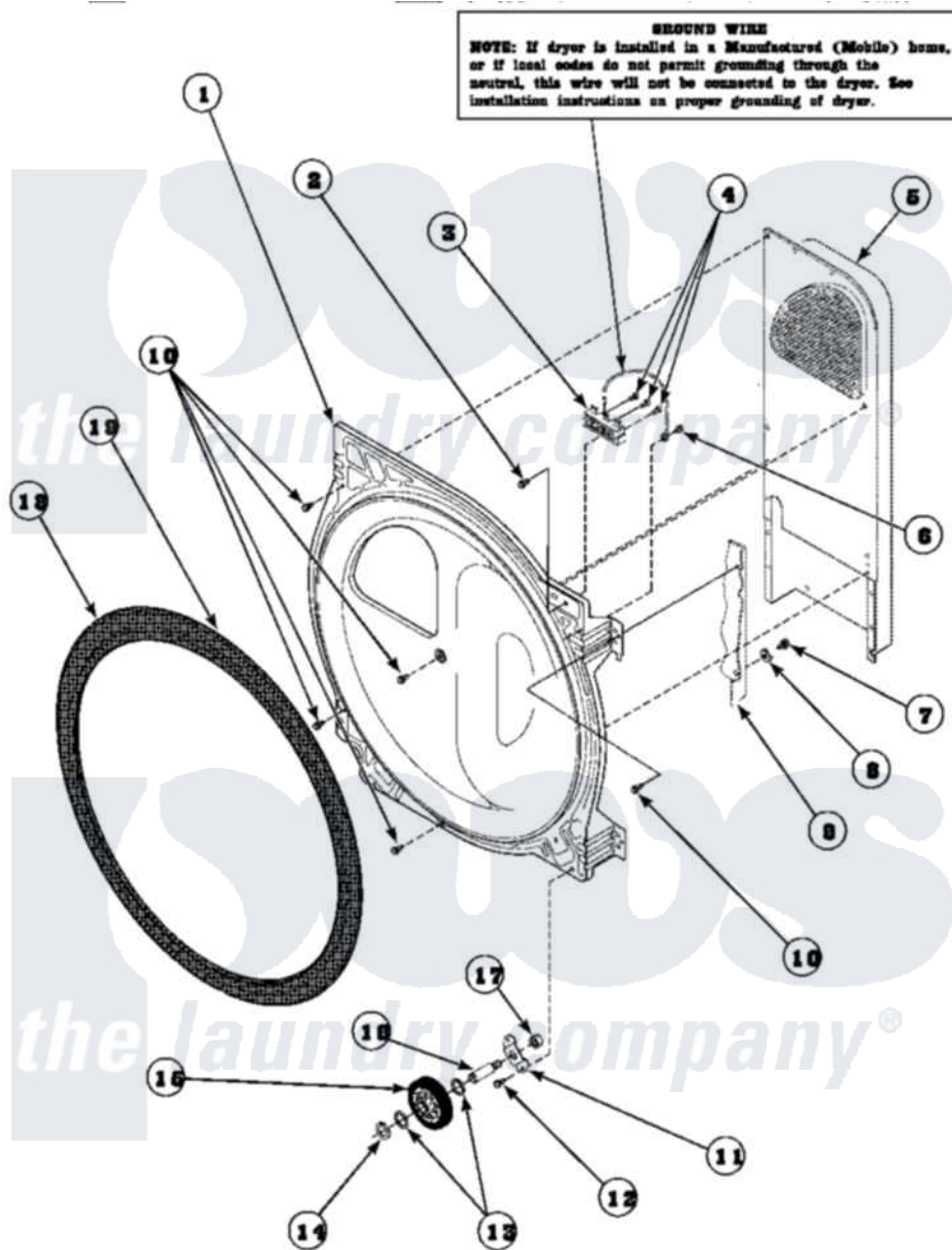
Amana Residential Amana LE8467W2 (BOM: PLE8467W2) Dryer Parts Parts Diagram 16 - REAR BLKHD/FELT SEAL/CYL ROLLER & TERM Click on the part number to view part
