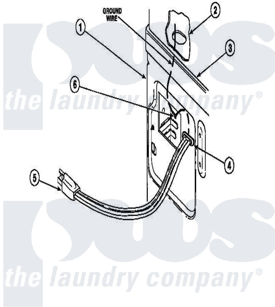
Amana Residential Amana LE8517L2 (BOM: PLE8517L2) Dryer Parts Parts Diagram 18 - POWER CORDS Click on the part number to view part
