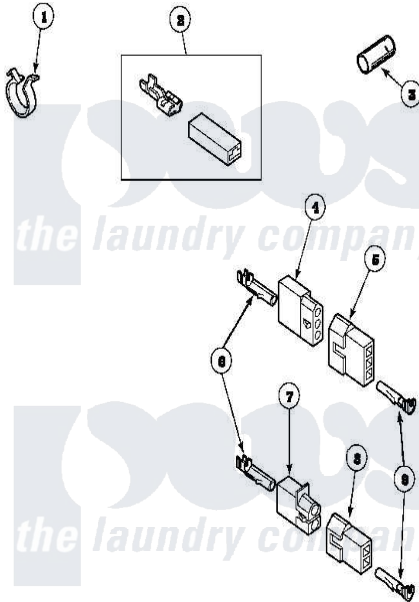
Amana Residential Amana LE8517W2B (BOM: PLE8517W2 B) Dryer Parts Parts Diagram 13 - TERMINALS Click on the part number to view part
