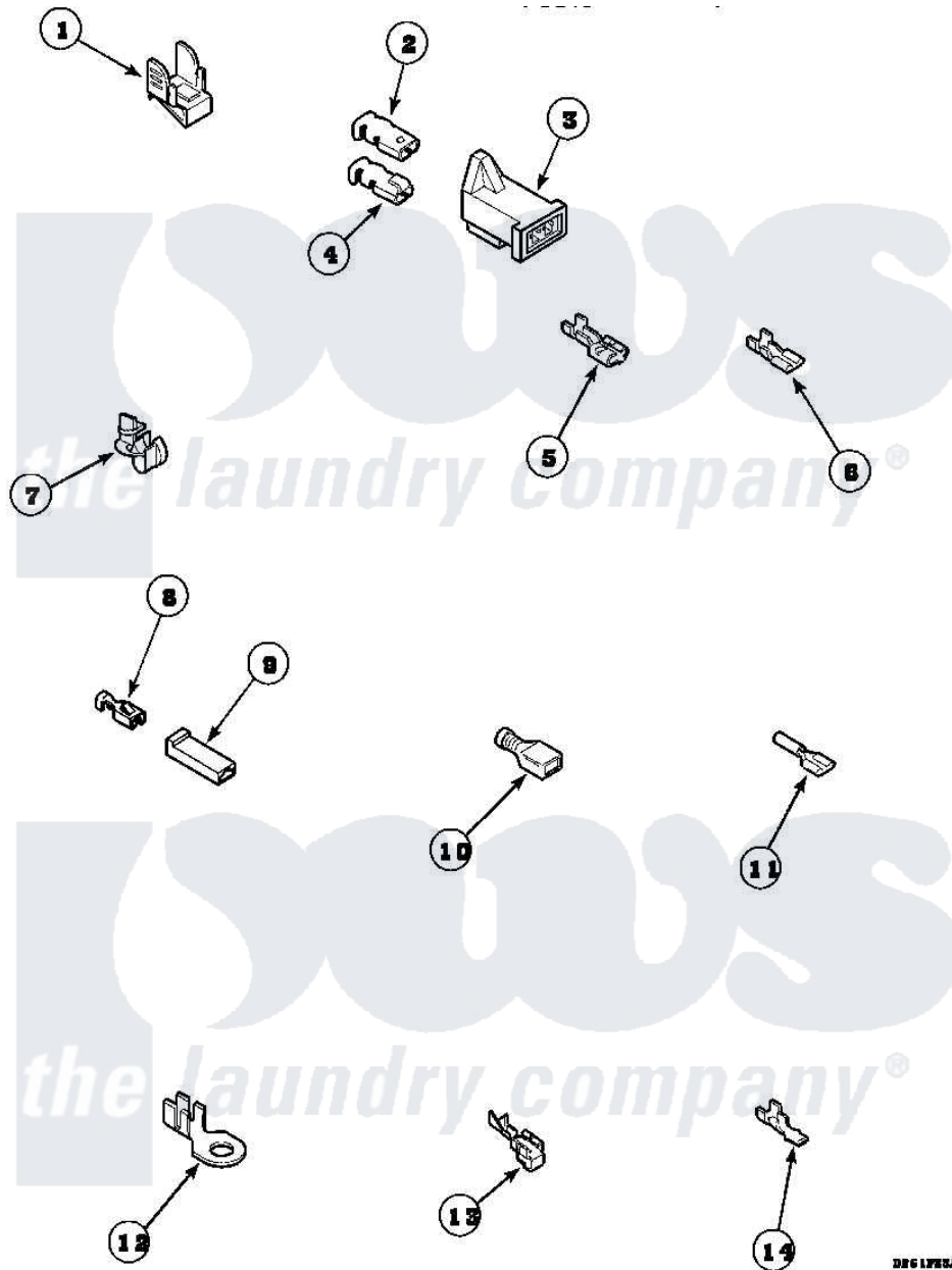
Amana Residential Amana LE8517W2B (BOM: PLE8517W2 B) Dryer Parts Parts Diagram 14 - TERMINALS Click on the part number to view part
