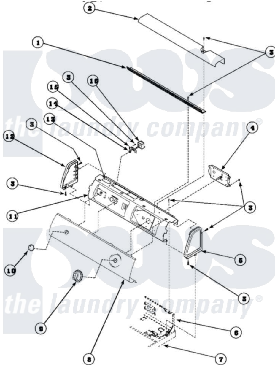
Amana Residential Amana LE8567L2 (BOM: PLE8567L2) Dryer Parts Parts Diagram 07 - GRAPHIC PANEL, CONTROL HOOD AND CONTROLS
