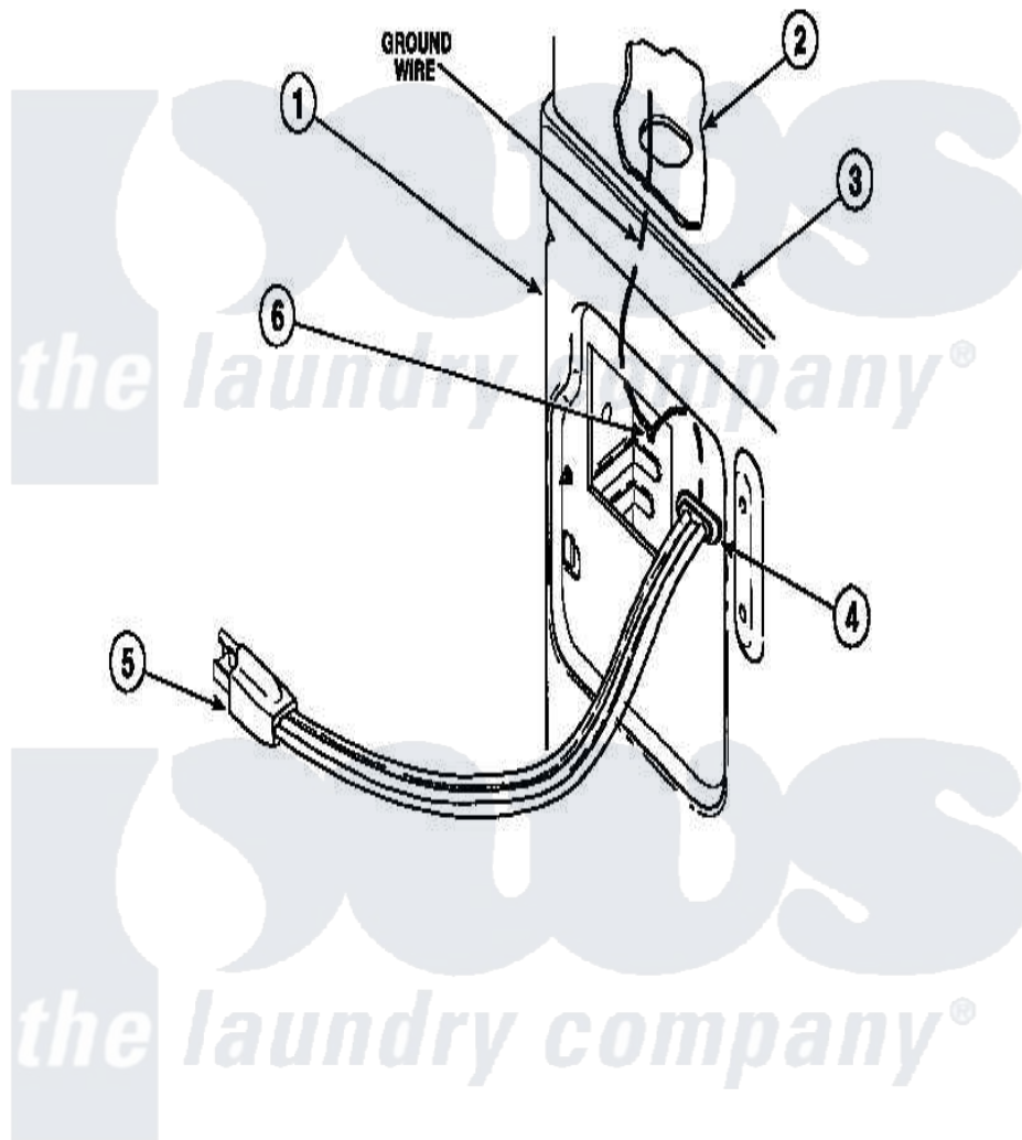
Amana Residential Amana LE8607W2 (BOM: PLE8607W2) Dryer Parts Parts Diagram 18 - POWER CORDS Click on the part number to view part
