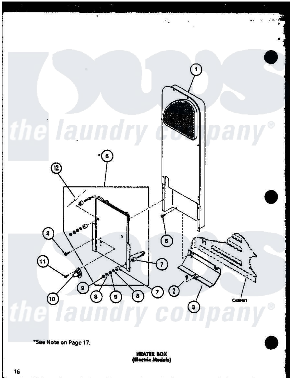
Amana Residential Amana LE9002 (BOM: P7804821W) Dryer Parts Diagram 03 - HEATER BOX (ELECTRIC MODELS)
