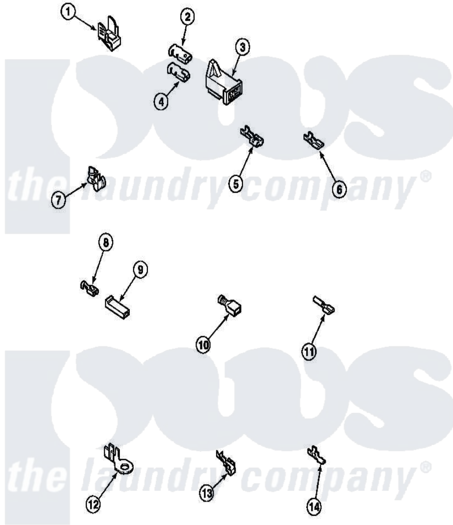
Amana Residential Amana LE9207W2 (BOM: PLE9207W2) Dryer Parts Parts Diagram 21 - TERMINALS
