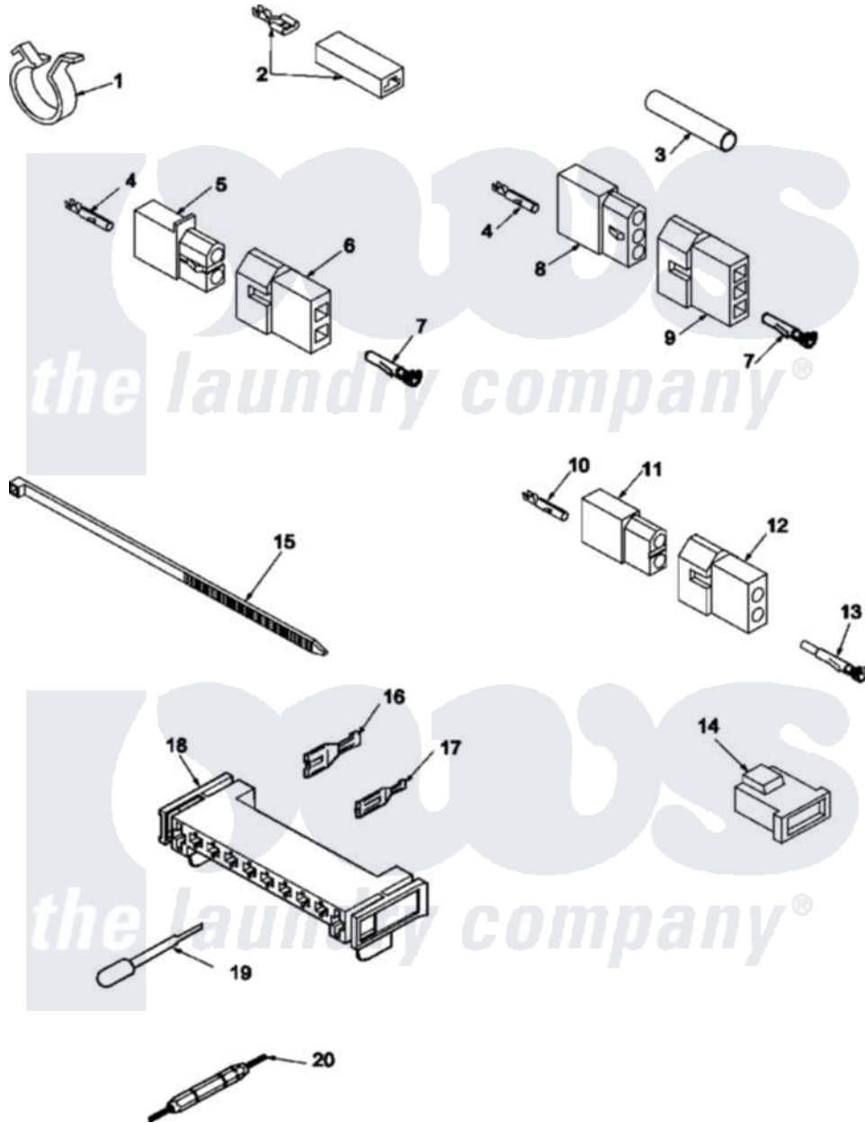
Amana Residential Amana LEA90AW (BOM: PLEA90AW) Dryer Parts Parts Diagram 09 - TERMINALS AND MOTOR CONNECTION BLOCK
