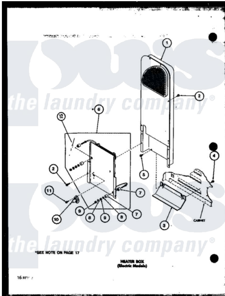
Amana Residential Amana LED250 (BOM: P7762207W) Washer Parts Parts Diagram 03 - HEATER BOX (ELECTRIC MODELS)
