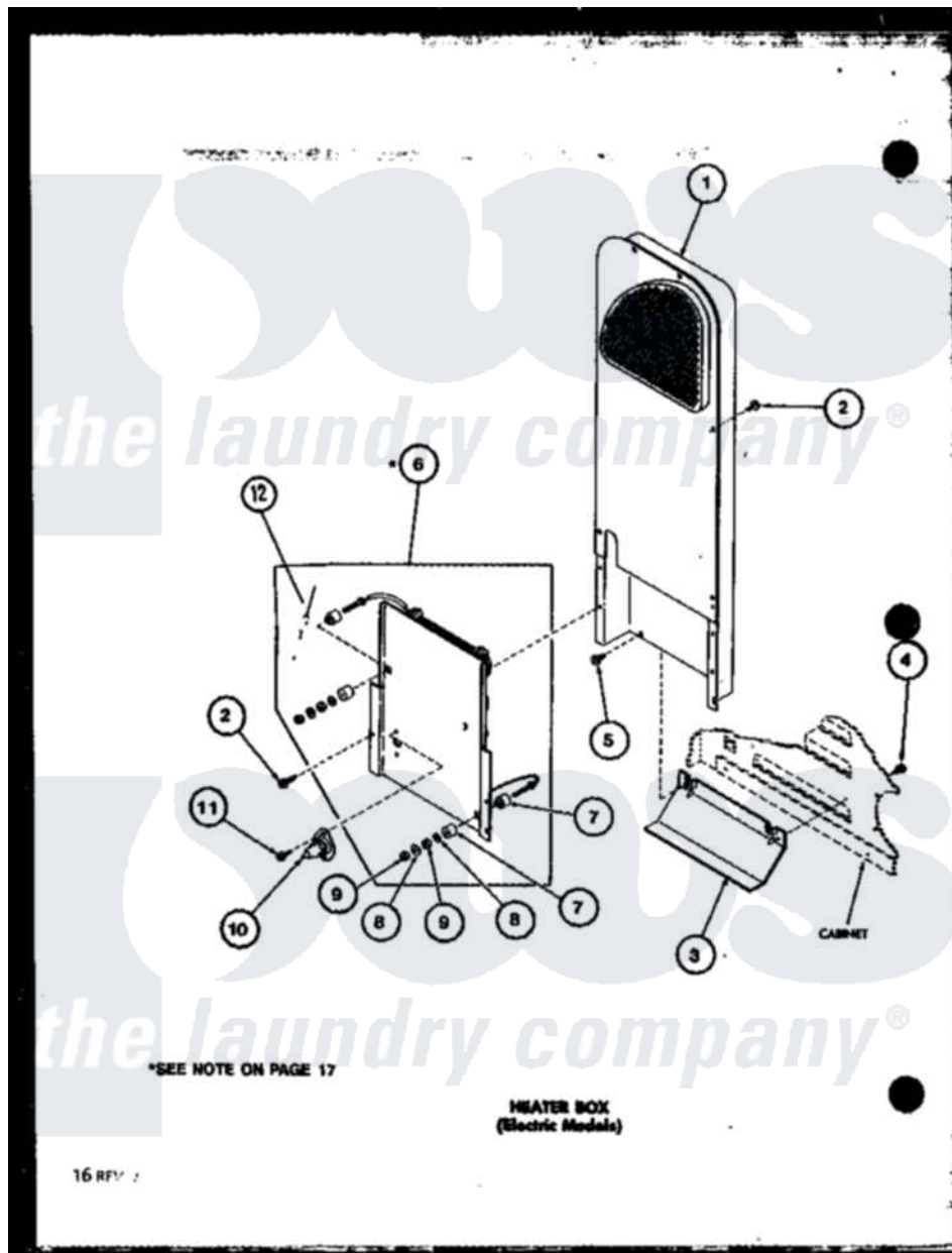
Amana Residential Amana LED250 (BOM: P7762231W) Dryer Parts Parts Diagram 03 - HEATER BOX (ELECTRIC MODELS)
