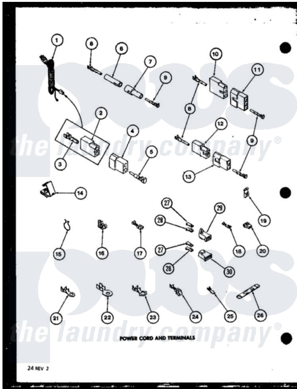
Amana Residential Amana LED450 (BOM: P7762209W) Washer Parts Parts Diagram 07 - POWER CORD AND TERMINALS
