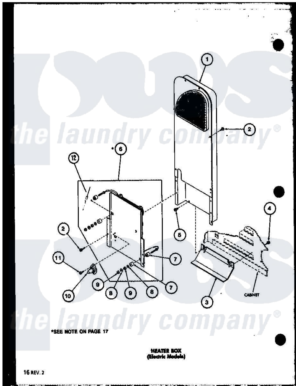
Amana Residential Amana LED450 (BOM: P7762233W) Dryer Parts Parts Diagram 03 - HEATER BOX (ELECTRIC MODELS)
