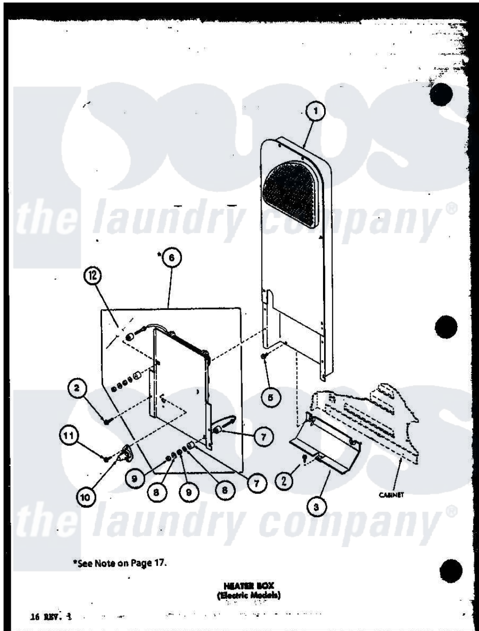
Amana Residential Amana LED502 (BOM: P7762223W) Dryer Parts Parts Diagram 03 - HEATER BOX (ELECTRIC MODELS)
