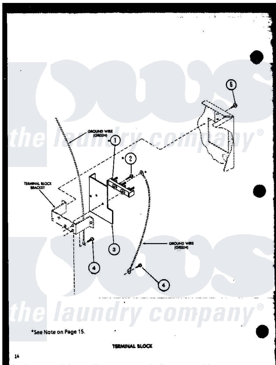
Amana Residential Amana LED502 (BOM: P7762223W) Dryer Parts Parts Diagram 08 - TERMINAL BLOCK Click on the part number to view part
