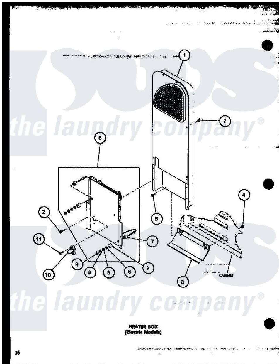
Amana Residential Amana LED850 (BOM: P7804805W) Washer Parts Parts Diagram 03 - HEATER BOX ( ELECTRIC MODELS)
