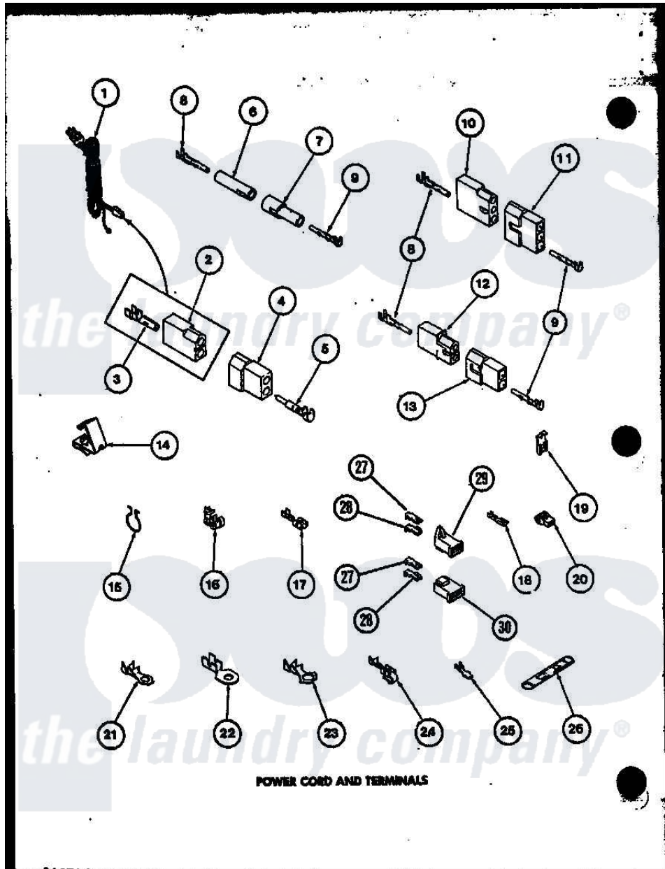
Amana Residential Amana LED850 (BOM: P7804809W) Dryer Parts Parts Diagram 07 - POWER CORD AND TERMINALS
