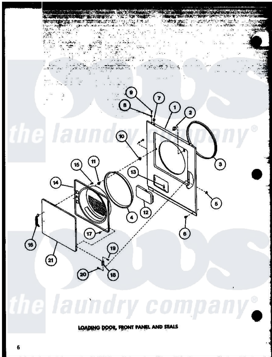
Amana Residential Amana LED902 (BOM: P7804819W) Dryer Parts Parts Diagram 04 - LOADING DOOR Click on the part number to view part
