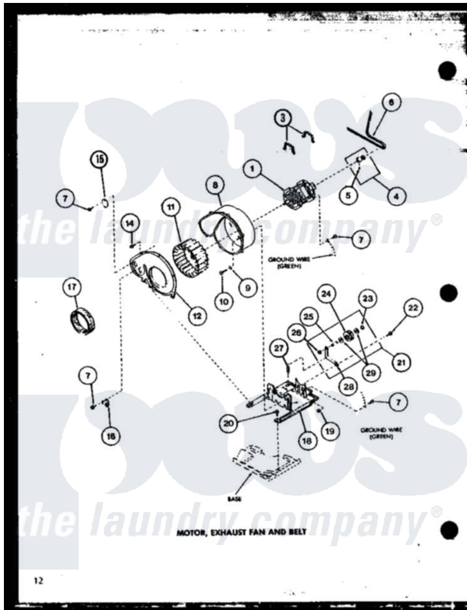
Amana Residential Amana LED902 (BOM: P7804819W) Dryer Parts Parts Diagram 05 - MOTOR
