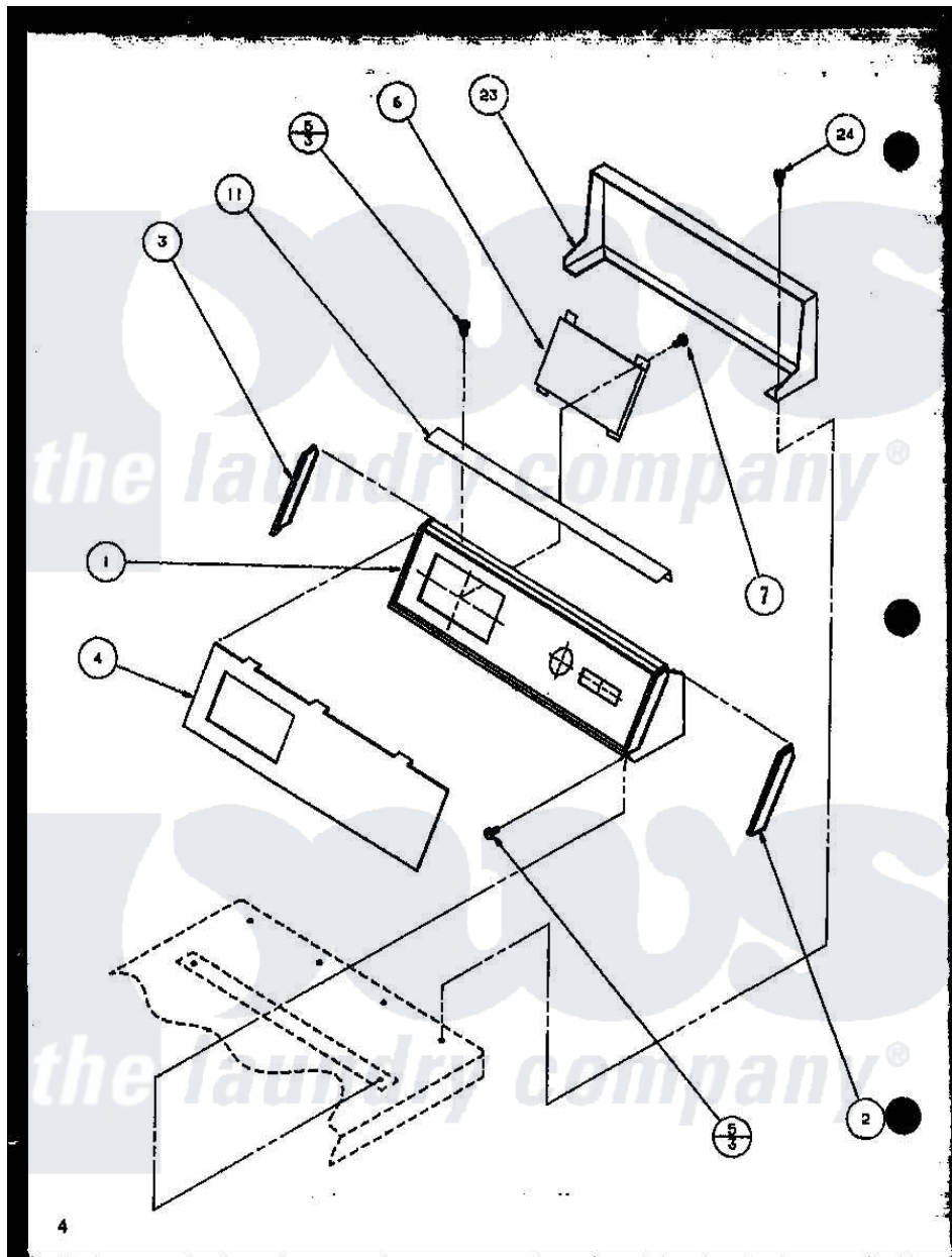
Amana Residential Amana LED902 (BOM: P7804819W) Dryer Parts Parts Diagram 06 - Page 1 Click on the part number to view part
