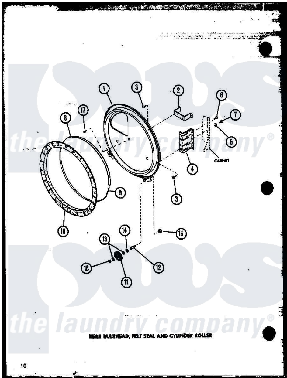
Amana Residential Amana LED902 (BOM: P7804819W) Dryer Parts Parts Diagram 07 - REAR BULKHEAD Click on the part number to view part
