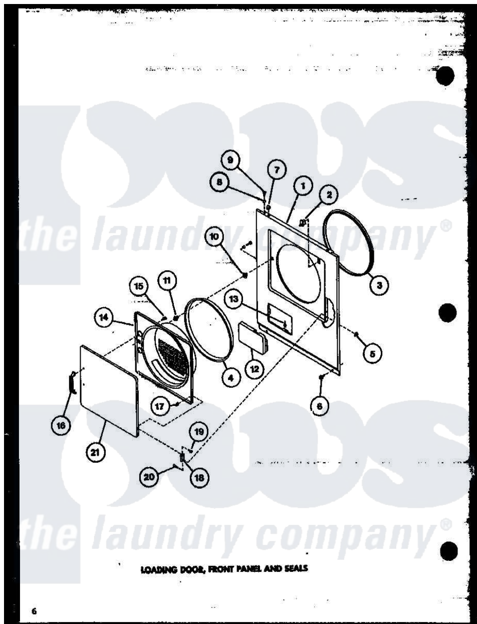
Amana Residential Amana LED950 (BOM: P7804807W) Washer Parts Parts Diagram 04 - LOADING DOOR Click on the part number to view part
