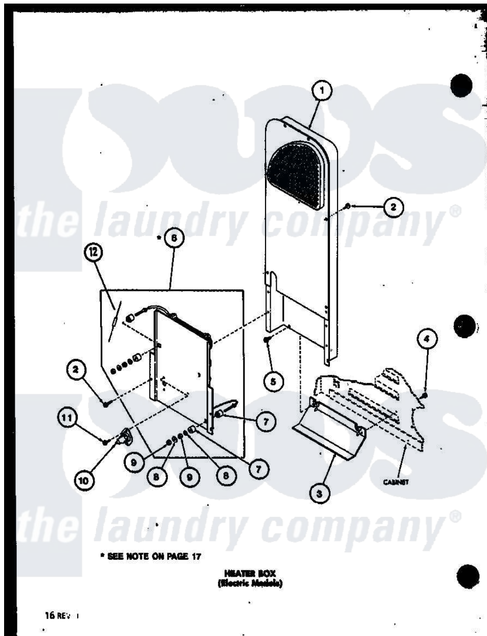
Amana Residential Amana LED950 (BOM: P7804827W) Dryer Parts Parts Diagram 03 - HEATER BOX (ELECTRIC MODELS)
