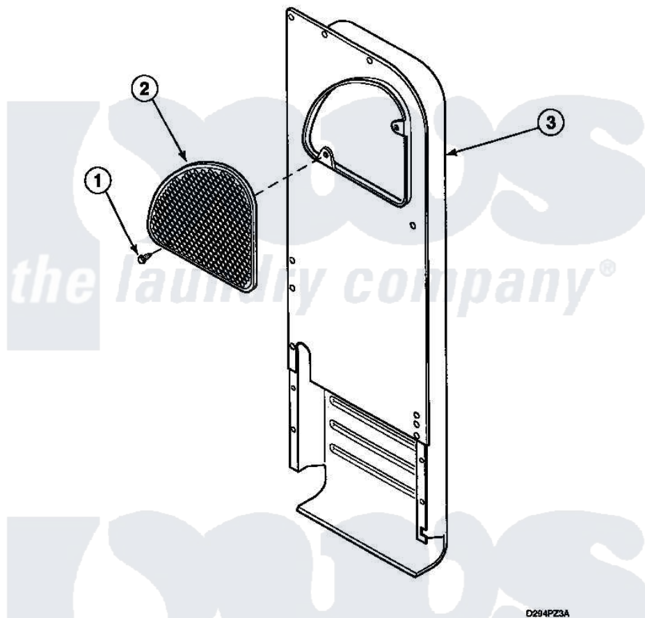
HEATER DUCT ASSEMBLY REPLACEMENT
