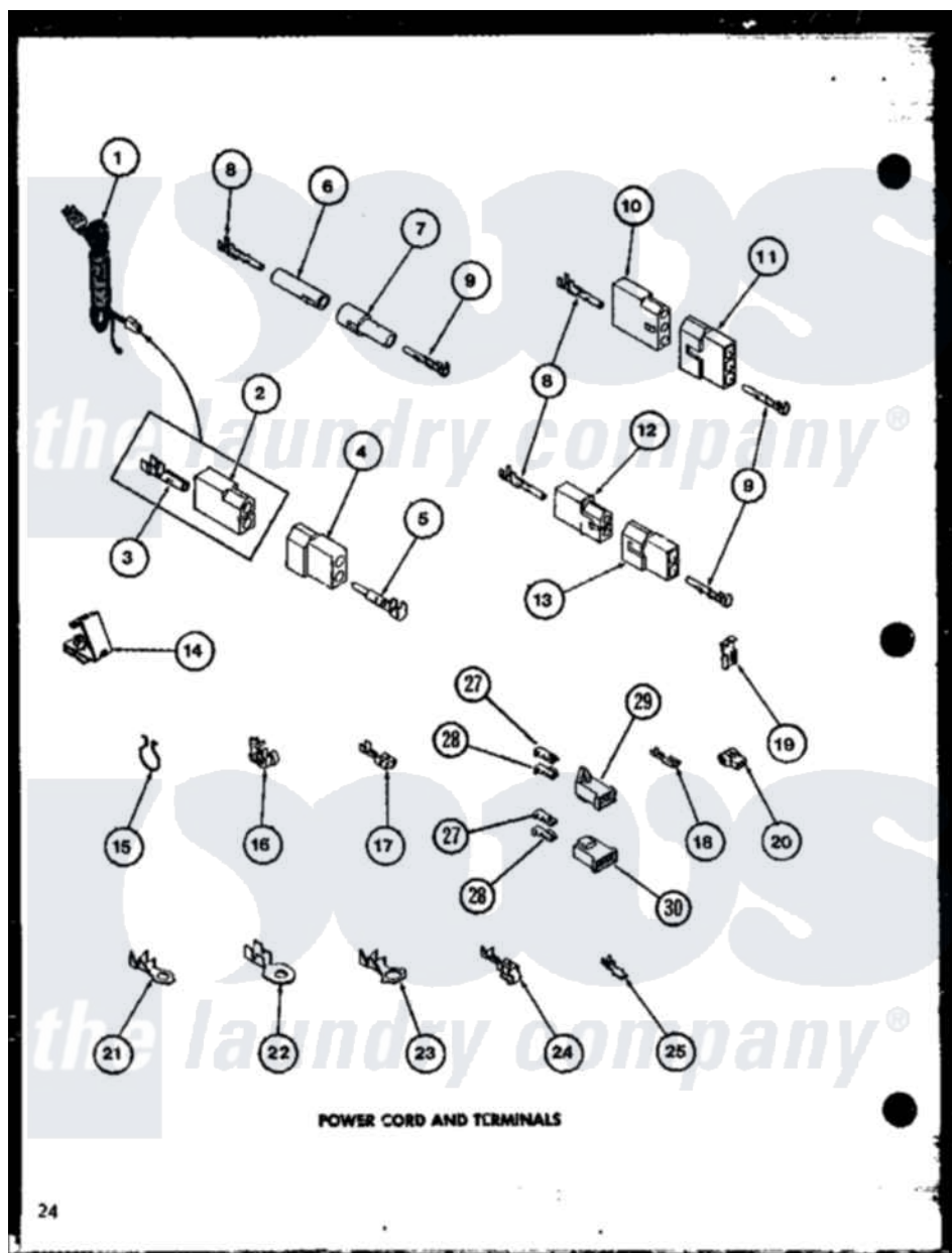
Amana Residential Amana LG1112 (BOM: P7762216W W) Washer Parts Parts Diagram 08 - POWER CORD AND TERMINALS
