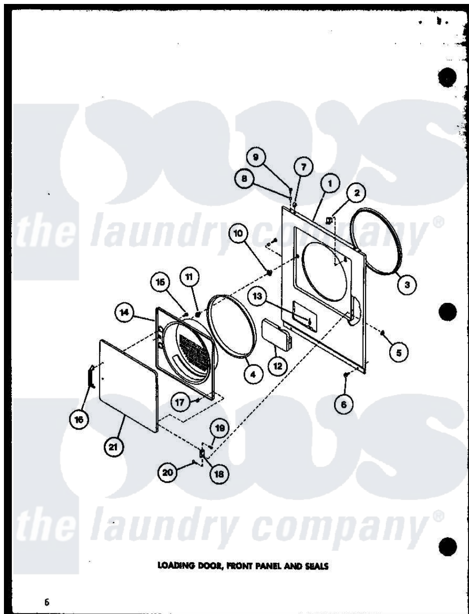
Amana Residential Amana LG1112 (BOM: P7762226W W) Dryer Parts Parts Diagram 04 - LOADING DOOR Click on the part number to view part
