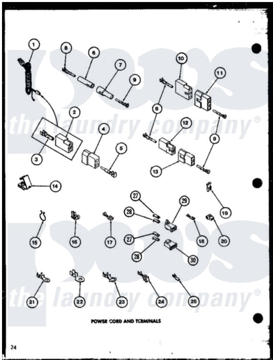
Amana Residential Amana LG2512 (BOM: P7762220W W) Washer Parts Parts Diagram 08 - POWER CORD AND TERMINALS
