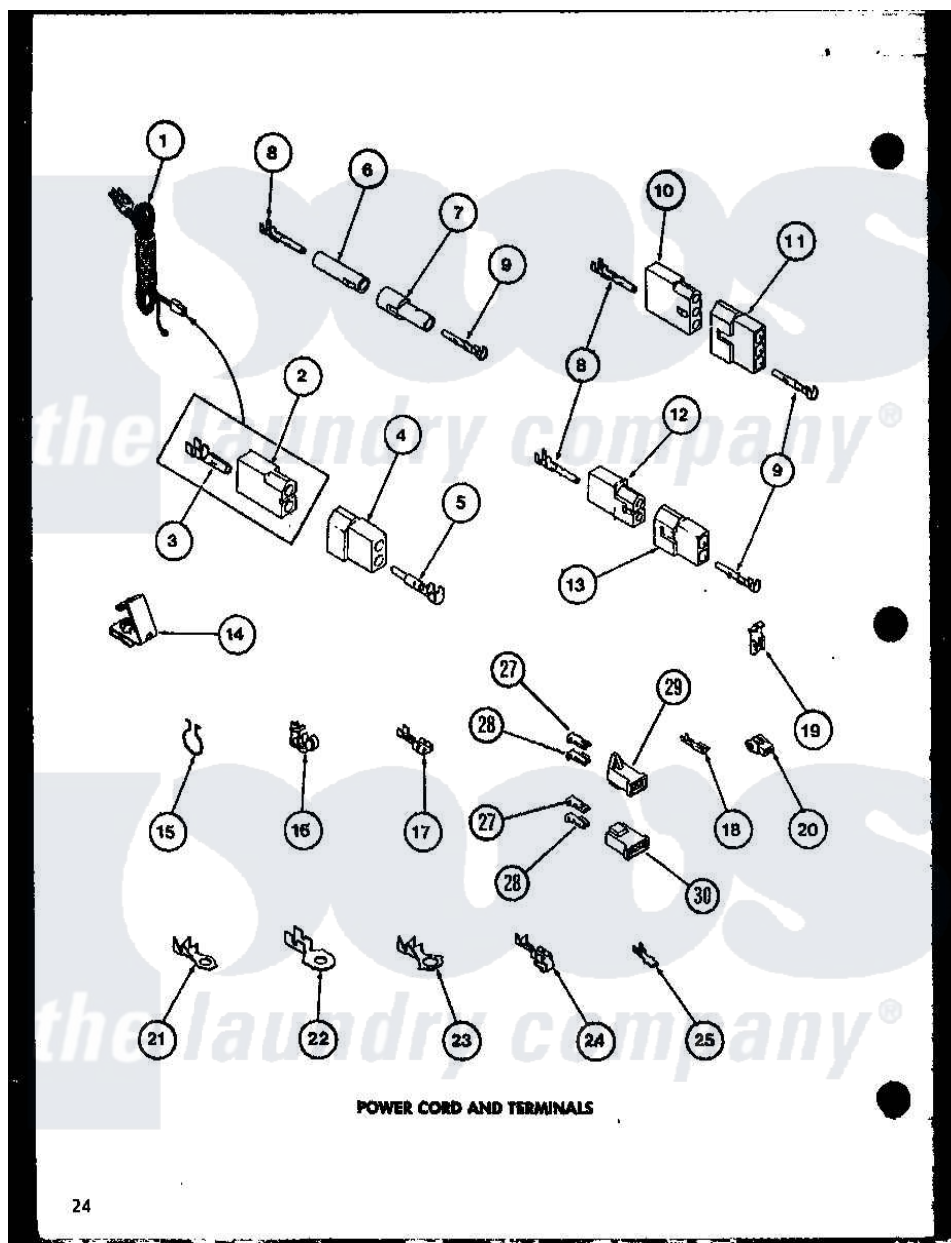
Amana Residential Amana LG2812 (BOM: P7804816W W) Washer Parts Parts Diagram 06 - POWER CORD AMD TERMINALS
