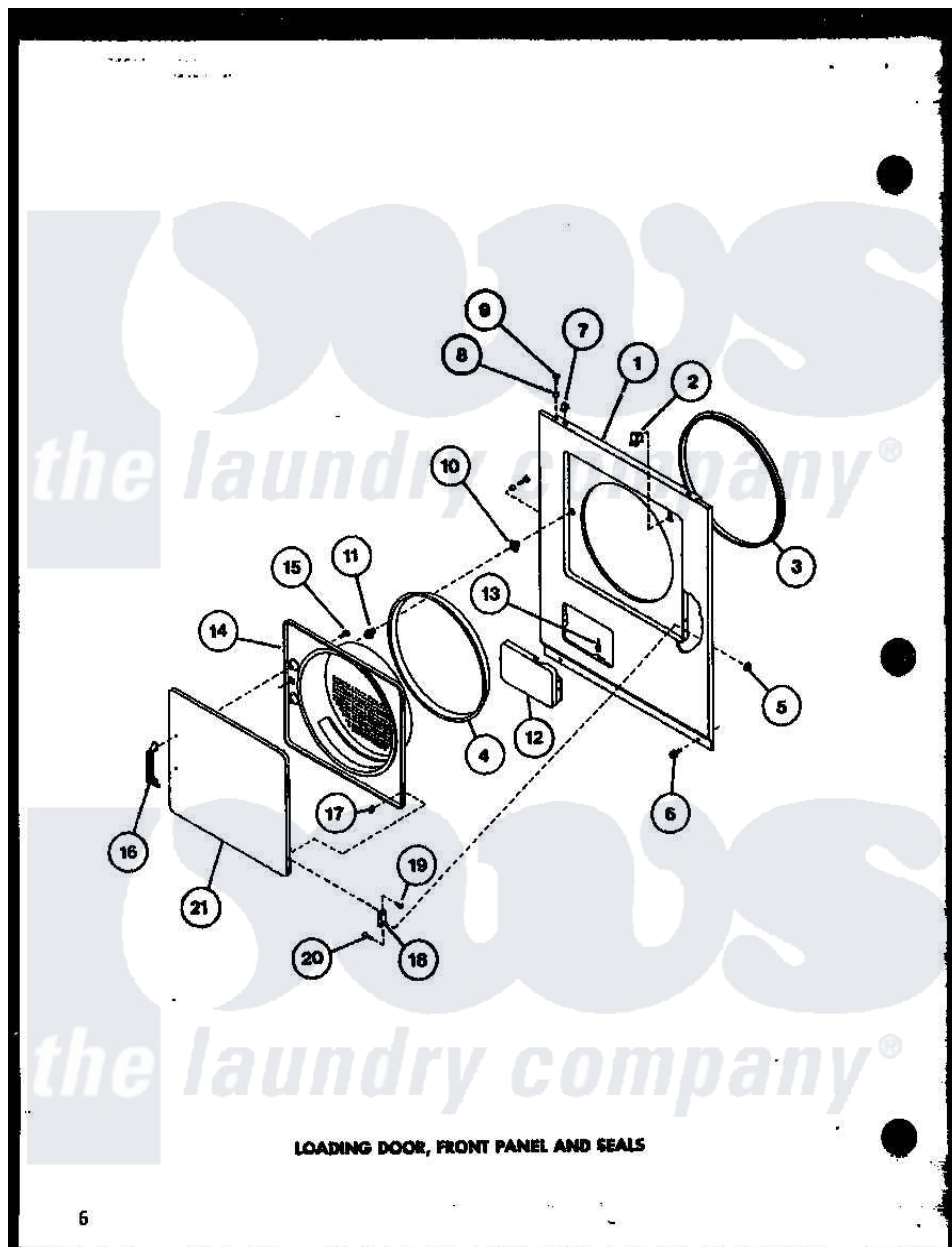
Amana Residential Amana LG2812 (BOM: P7804824W W) Dryer Parts Parts Diagram 04 - LOADING DOOR Click on the part number to view part
