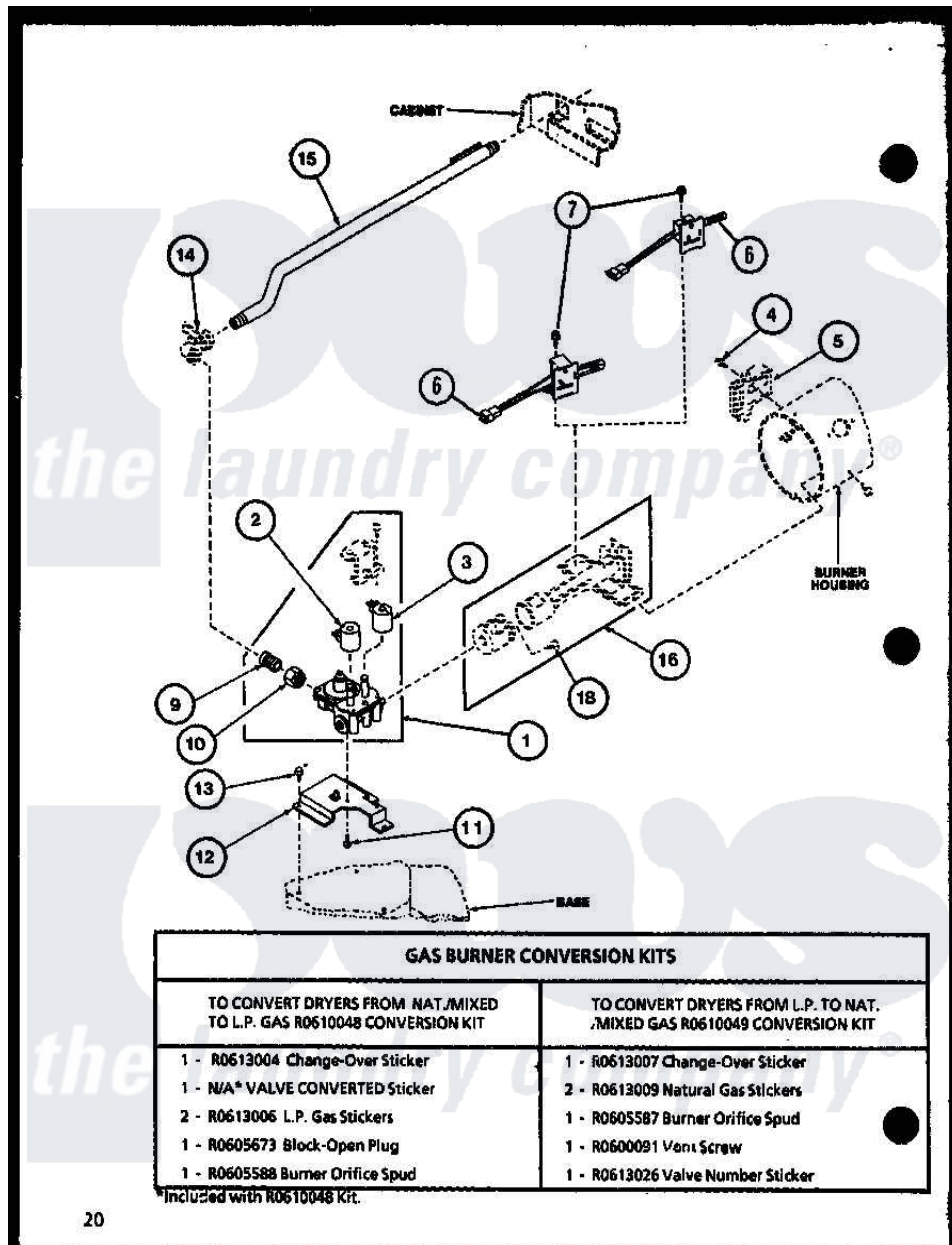
Amana Residential Amana LG2812 (BOM: P7804824W W) Dryer Parts Parts Diagram 07 - Page 9
