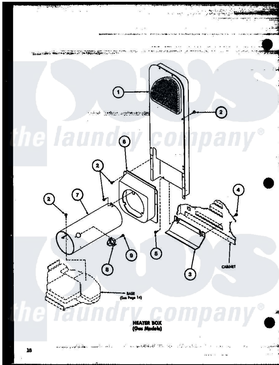
Amana Residential Amana LG2911 (BOM: P7804804W W) Dryer Parts Parts Diagram 03 - HEATER BOX (GAS MODELS)
