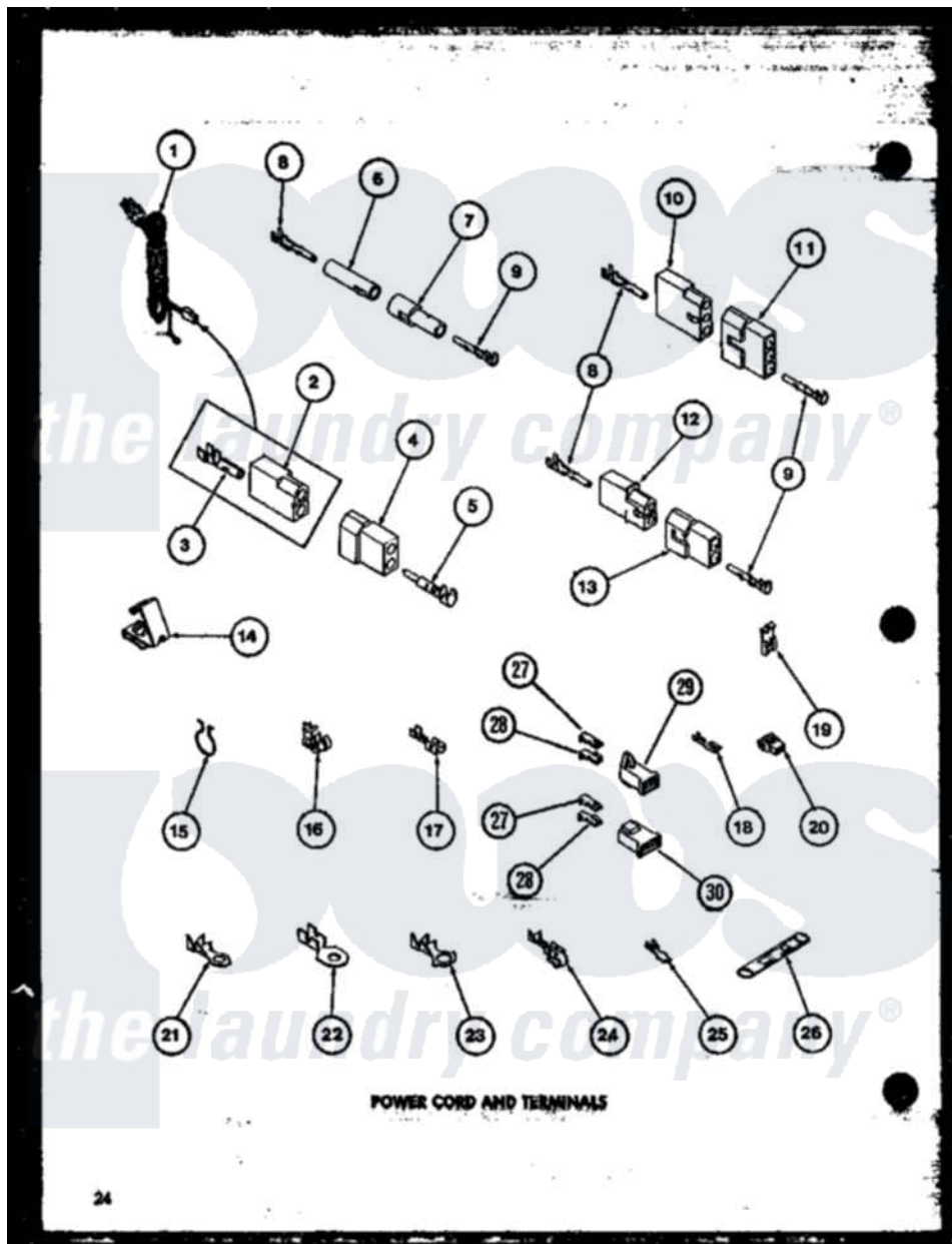
Amana Residential Amana LG2911 (BOM: P7804804W W) Dryer Parts Parts Diagram 08 - POWER CORD AND TERMINALS
