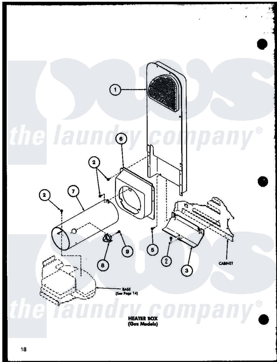
Amana Residential Amana LG2912 (BOM: P7804818W W) Washer Parts Parts Diagram 04 - HEATER BOX (GAS MODELS)
