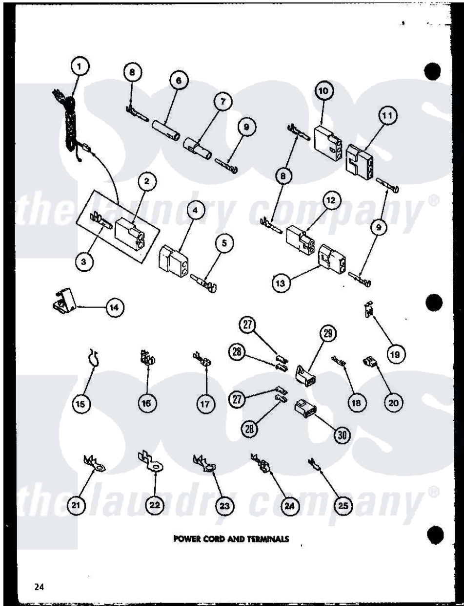
Amana Residential Amana LG2912 (BOM: P7804818W W) Washer Parts Parts Diagram 08 - POWER CORD AMD TERMINALS
