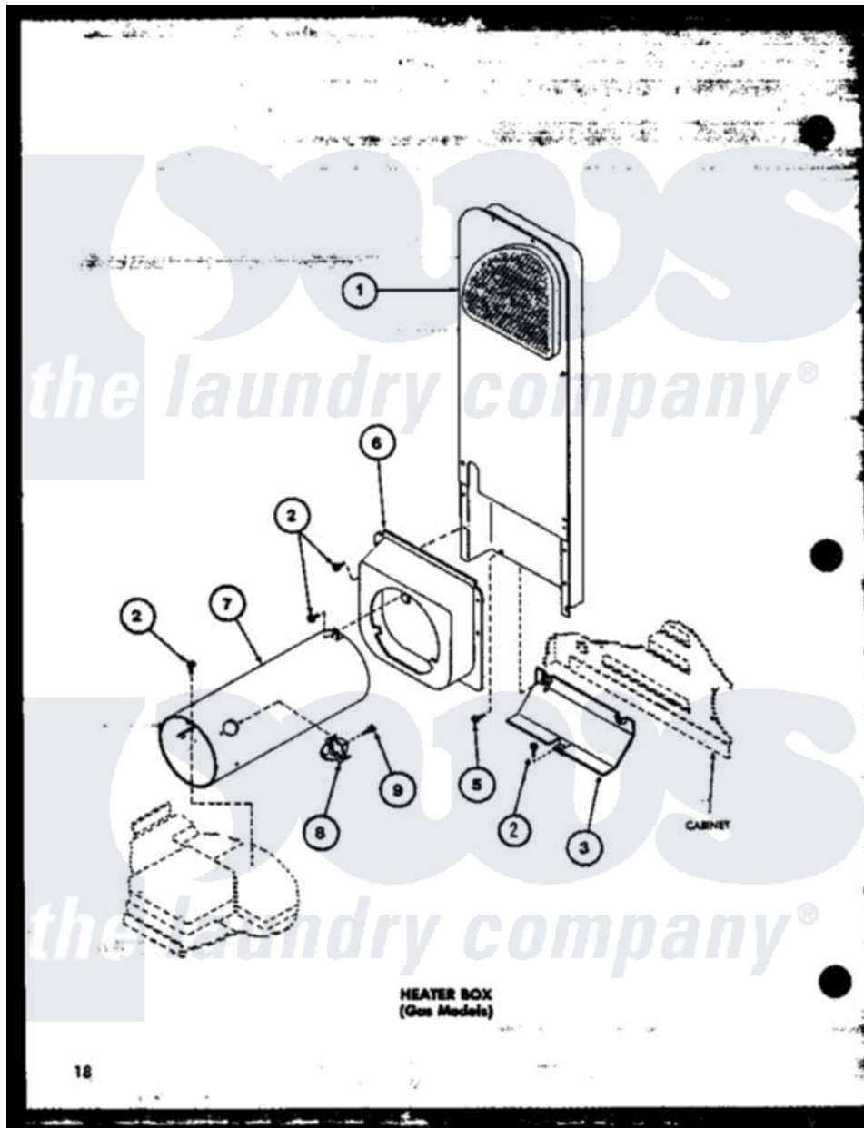
Amana Residential Amana LG3412G (BOM: P1122504W G) Dryer Parts Parts Diagram 04 - HEATER BOX (GAS MODELS)
