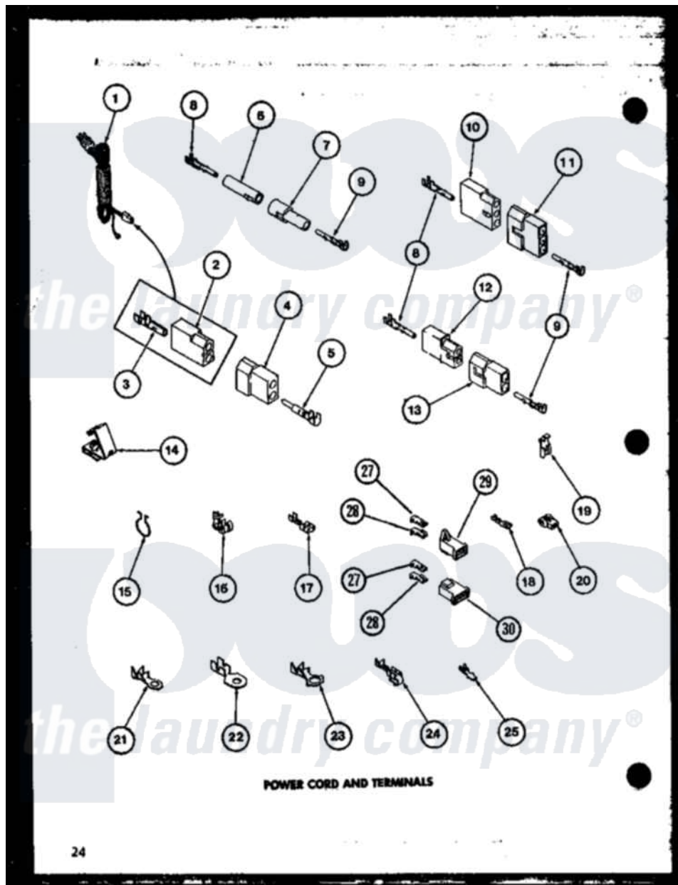
Amana Residential Amana LG3412W (BOM: P1122503W W) Dryer Parts Parts Diagram 08 - POWER CORD AND TERMINALS
