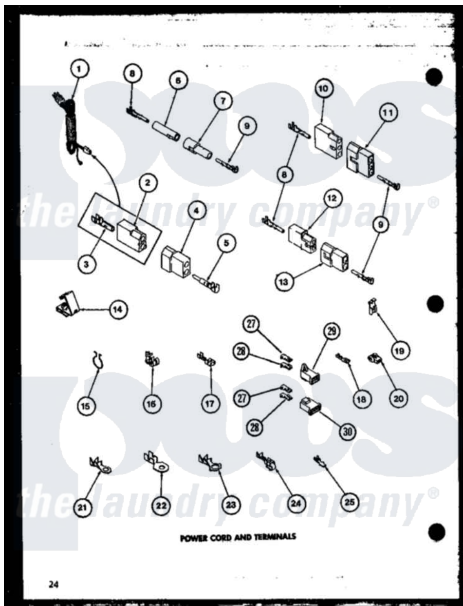
Amana Residential Amana LG3512W (BOM: P1122506W W) Dryer Parts Parts Diagram 08 - POWER CORD AND TERMINALS
